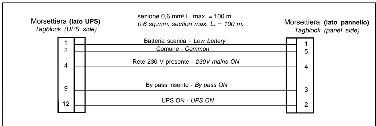
Fig. 2.6 - Schema del cavo di collegamento al Pannello remoto Drawing showing Remote Panel wiring cable
