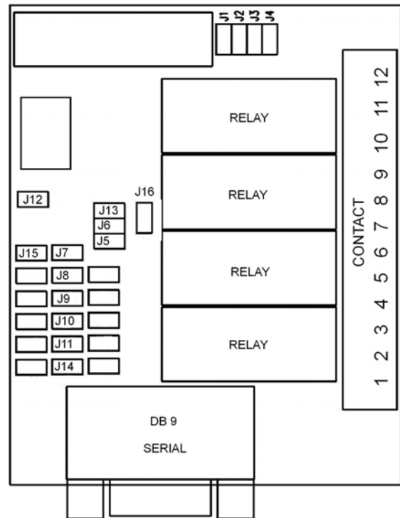
Ponticelli sulla scheda Relé Setting options on the Relay card
